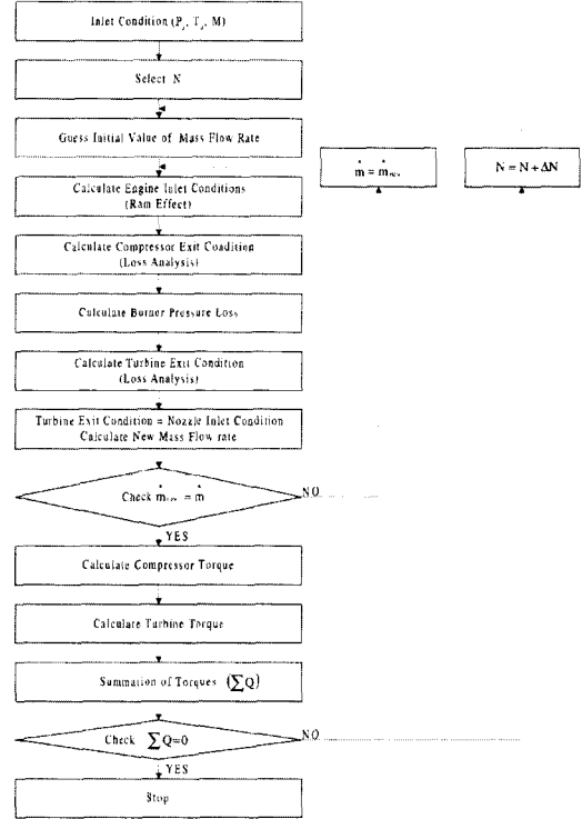
Fig. 3 Calculation process flow chart
