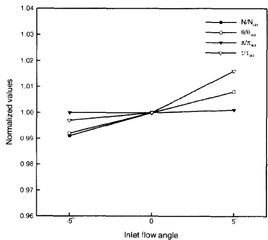
Fig. 11 The effect of inlet flow angle variation [ M=0.5 , ISA at 20,000 ft]
